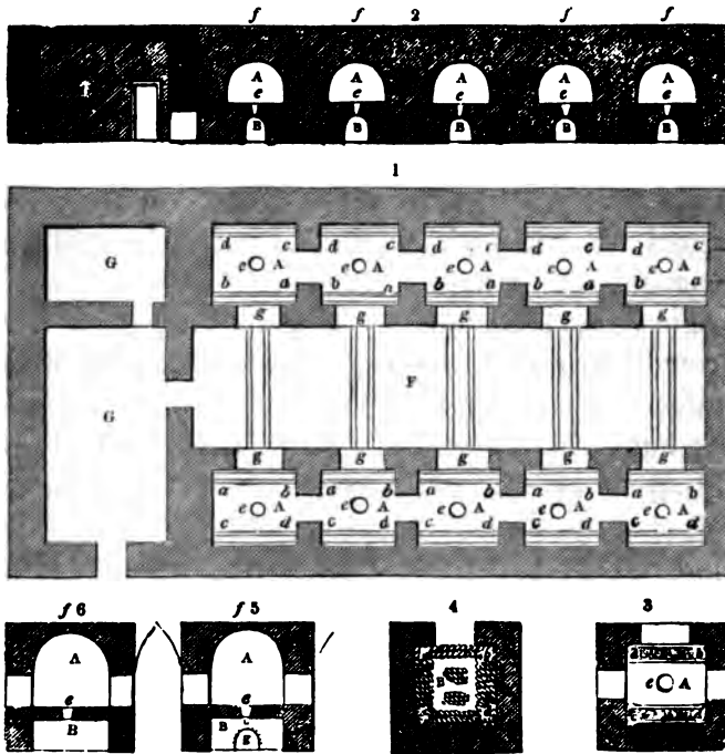
No. 443. Modern ovens for hatching eggs.
